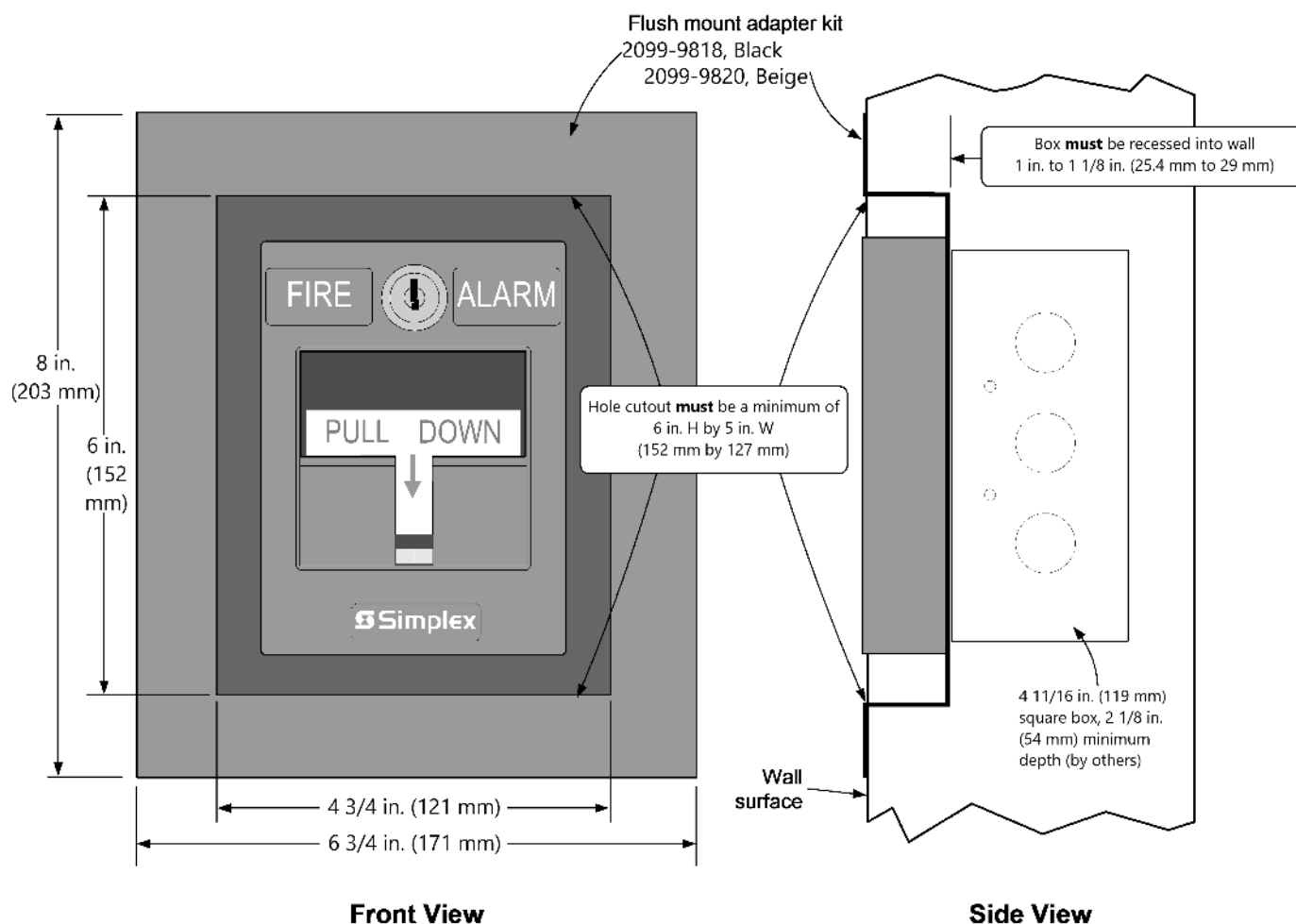
Figure 9: Flush mount reference
