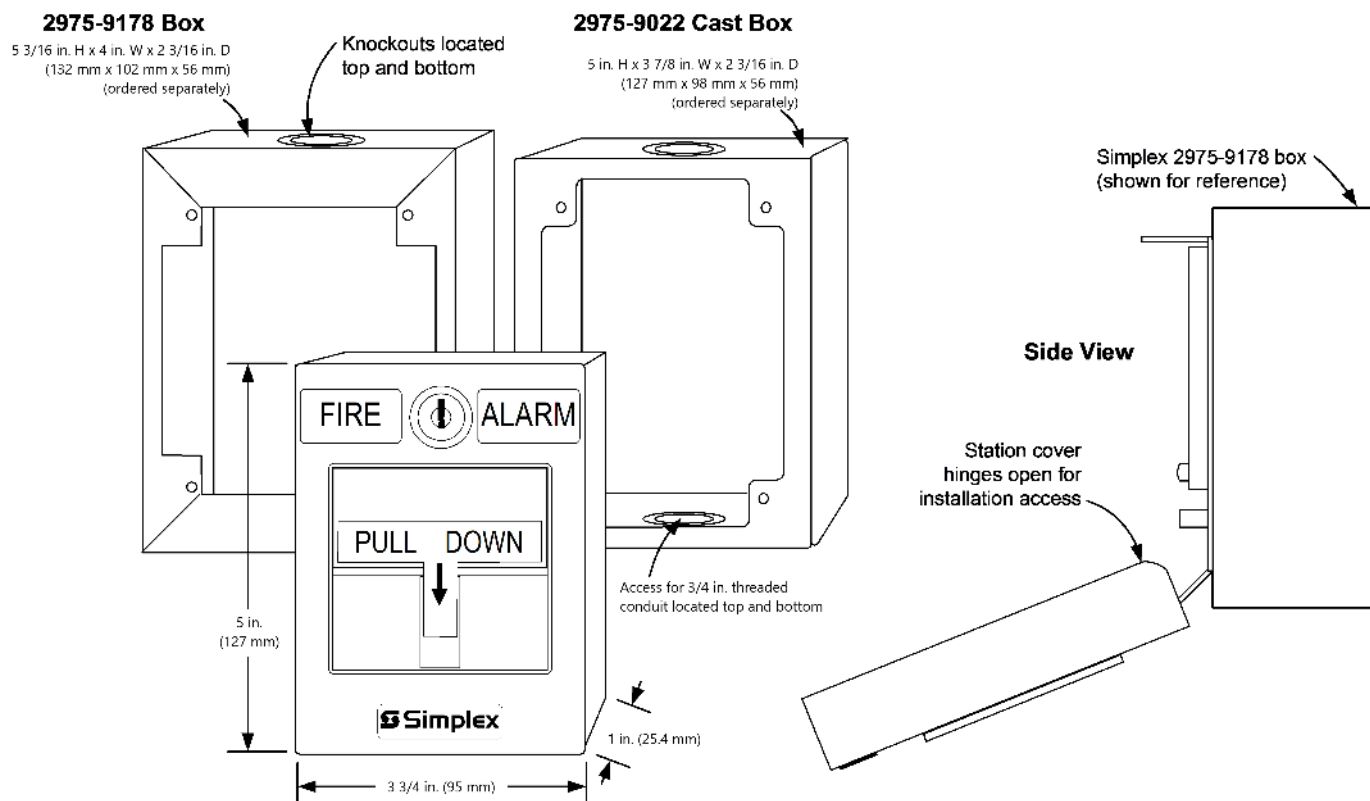
Figure 7: Surface mounting reference
