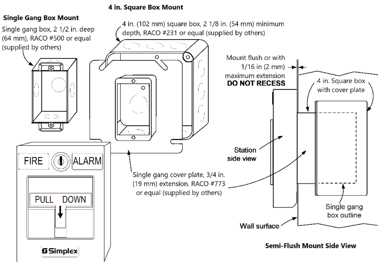
Figure 8: Semi-flush mounting reference
