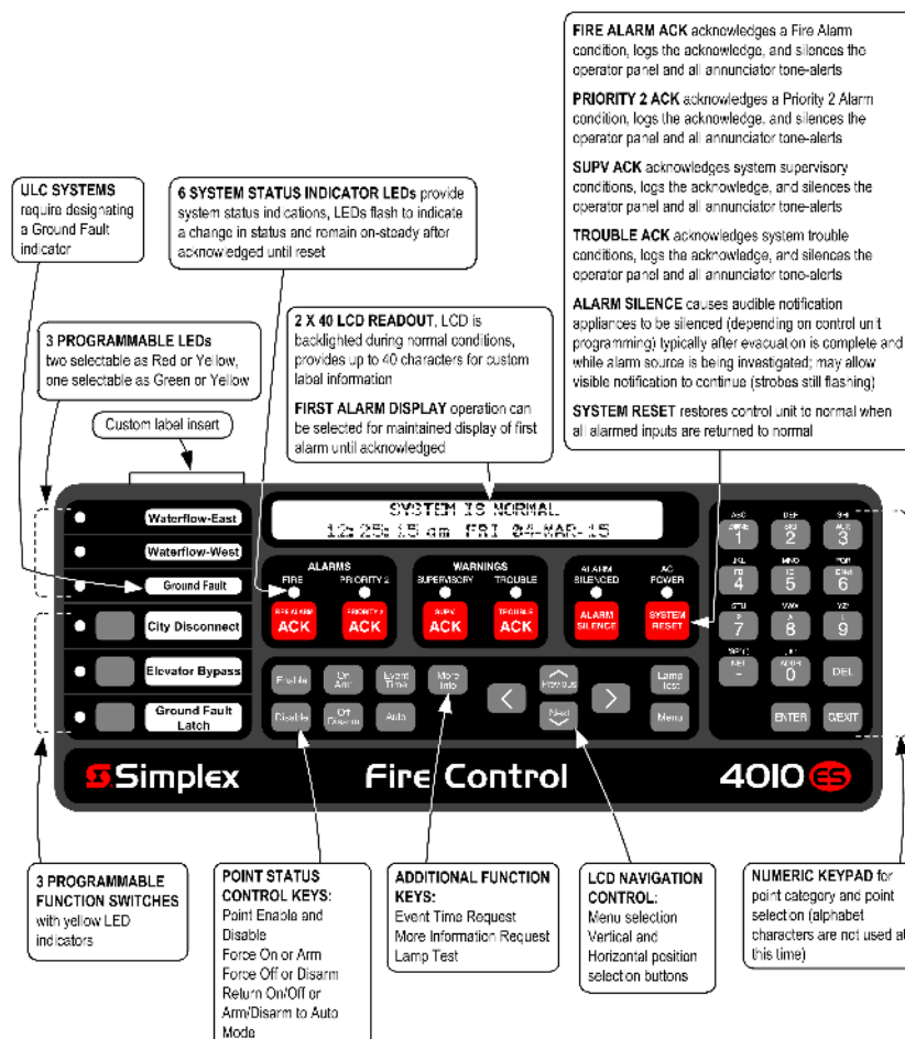
Figure 9: Operator interface features
