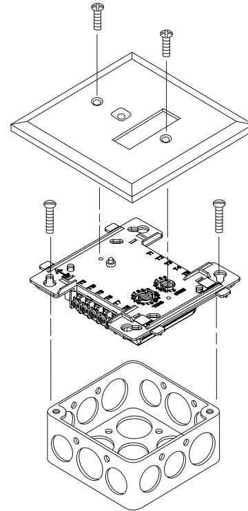
FIGURE 2. MODULE MOUNTING:
