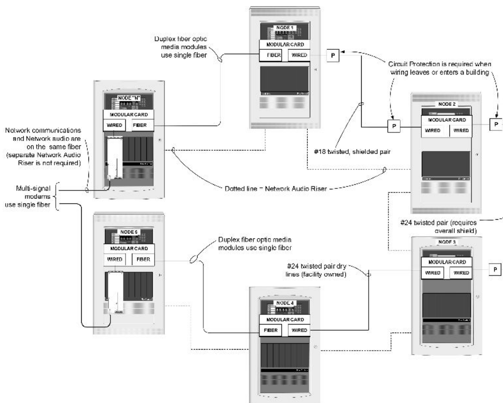
Figure 2: 4120 network communications options reference
