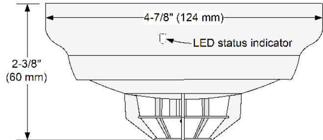
Figure 5: 4098-9733 Heat Sensor with Base
