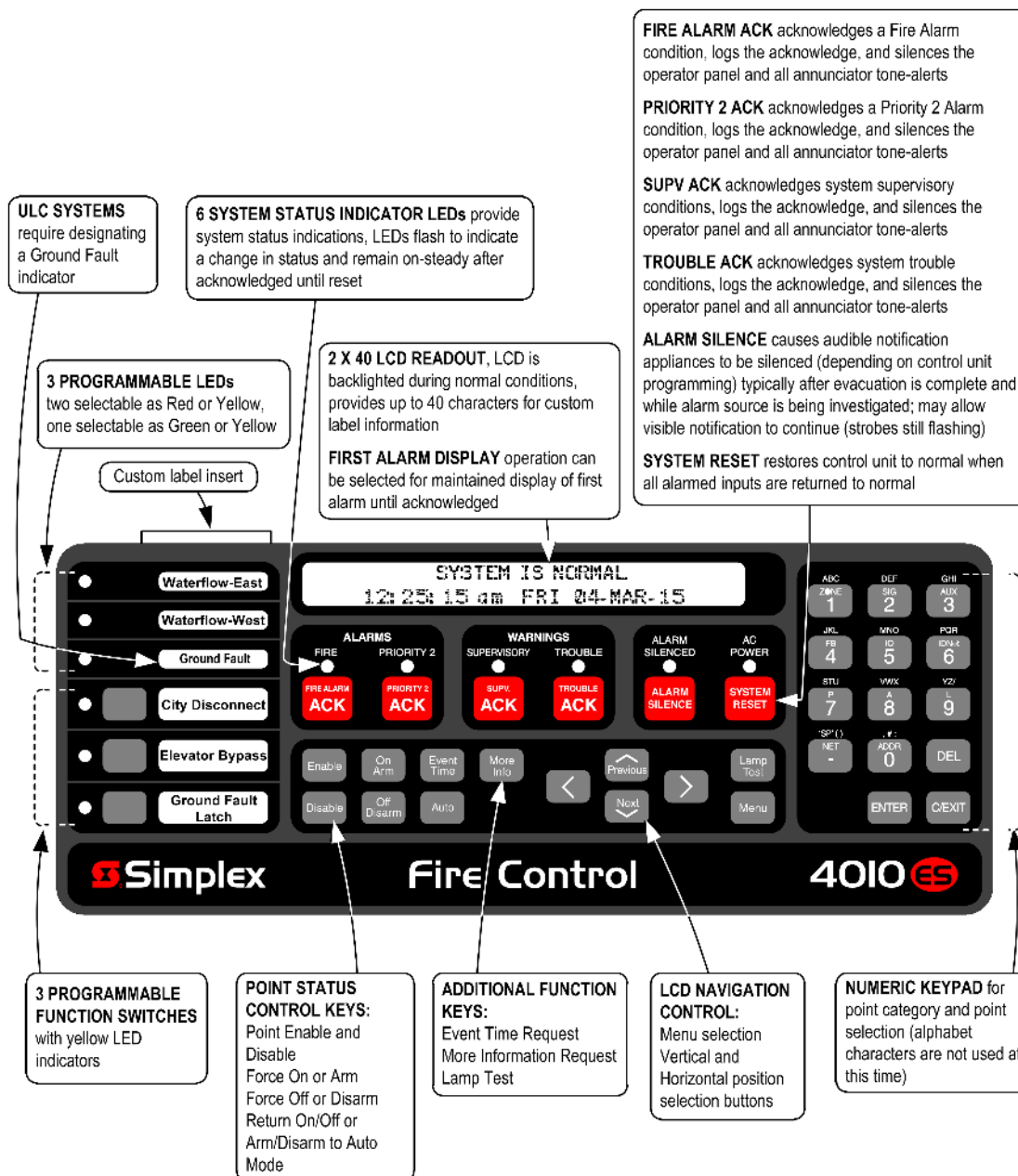
Figure 13: Operator Interface Features
