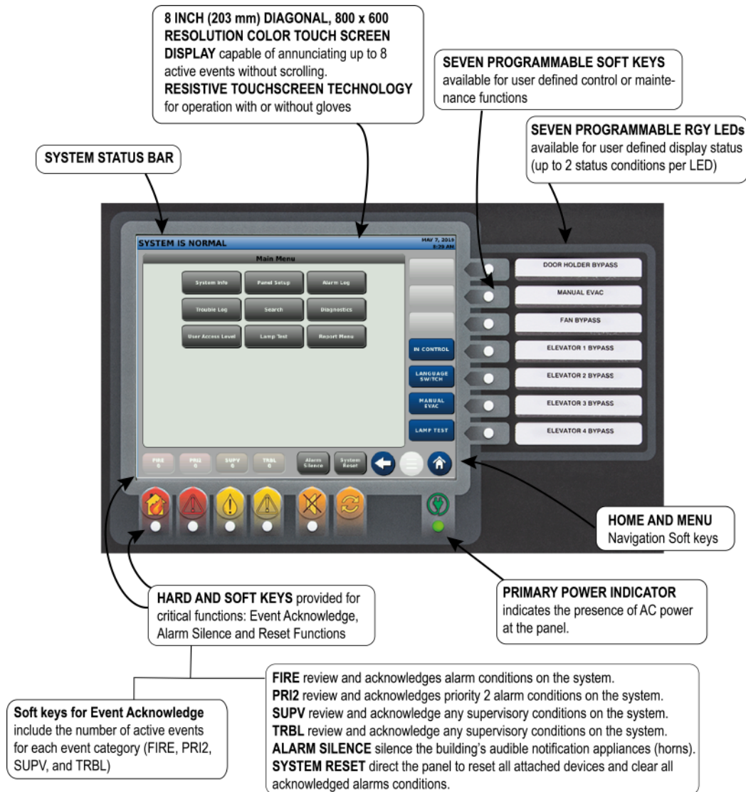
Figure 2: ES Touch Screen Display Operator Interface
