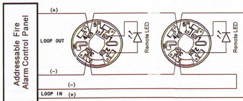
Figure 2. Typical wiring diagram
