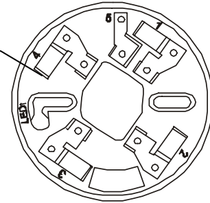
Figure 1. Terminal layout of HD10X base
